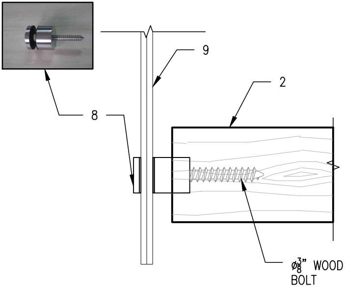
C STANDOFF WOOD CONN. DETAIL SD3.3 SCALE: 3"=1'-0"
