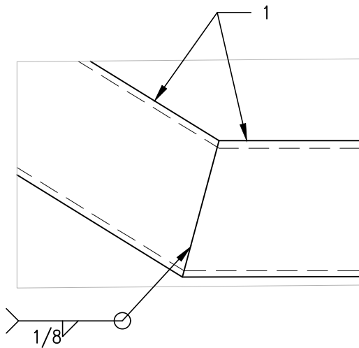
C TREAD DETAIL SD3.1 SCALE: 1 1/2"=1'-0"
