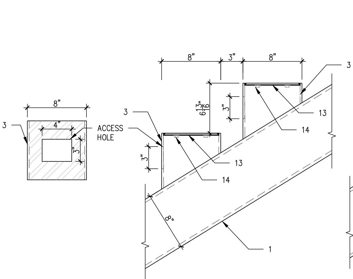
A TREAD DETAIL SD3.1 SCALE: 1 1/2"=1'-0"
