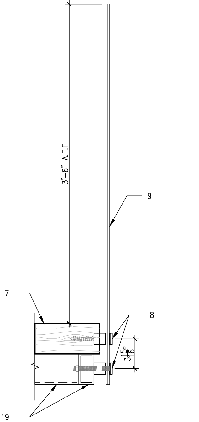
2 LANDING SECTION SD3.2 SCALE: 1 1/2"=1'-0"
